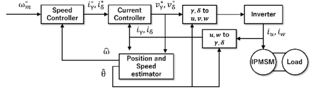
Fig. 8. System configuration of the sensorless control system for the IPMSM.
